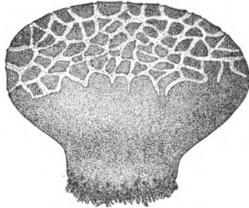
FIG. 336. — Lycoperdon cyathiforme : × \frac{1}{2} . (After Peck.)
